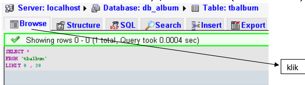
Gambar 12 Browse Tabel
