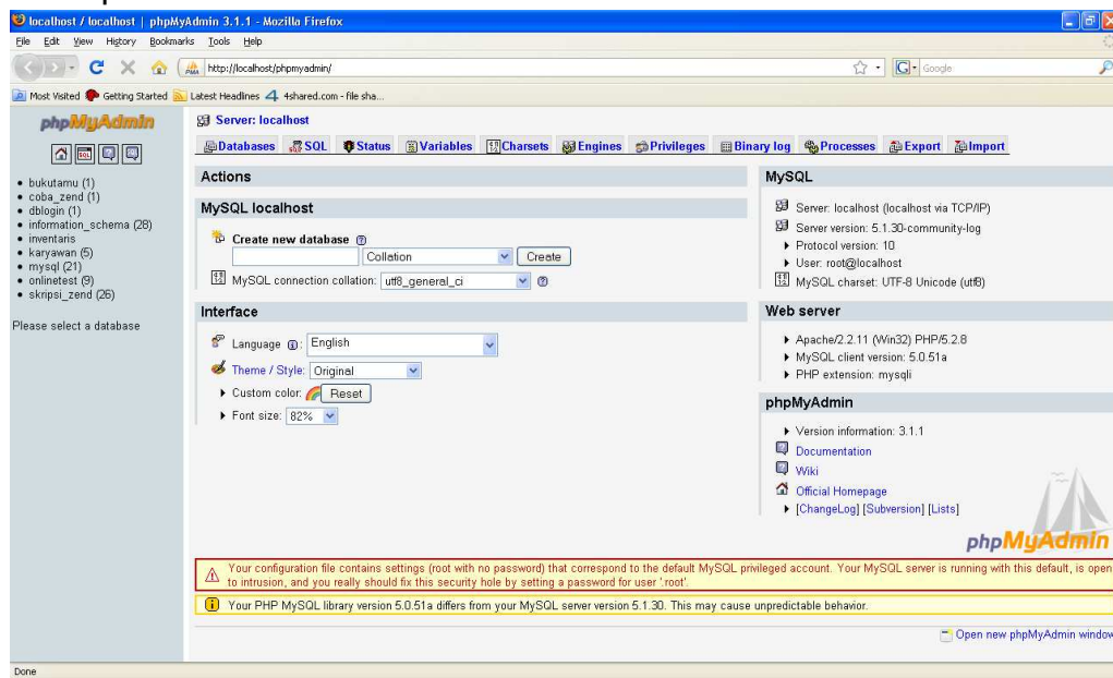
Gambar 5 Halaman phpMyAdmin
